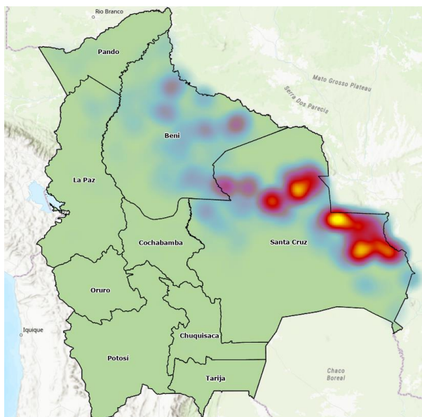
Heat map of fires in Bolivia Period: August 2024
