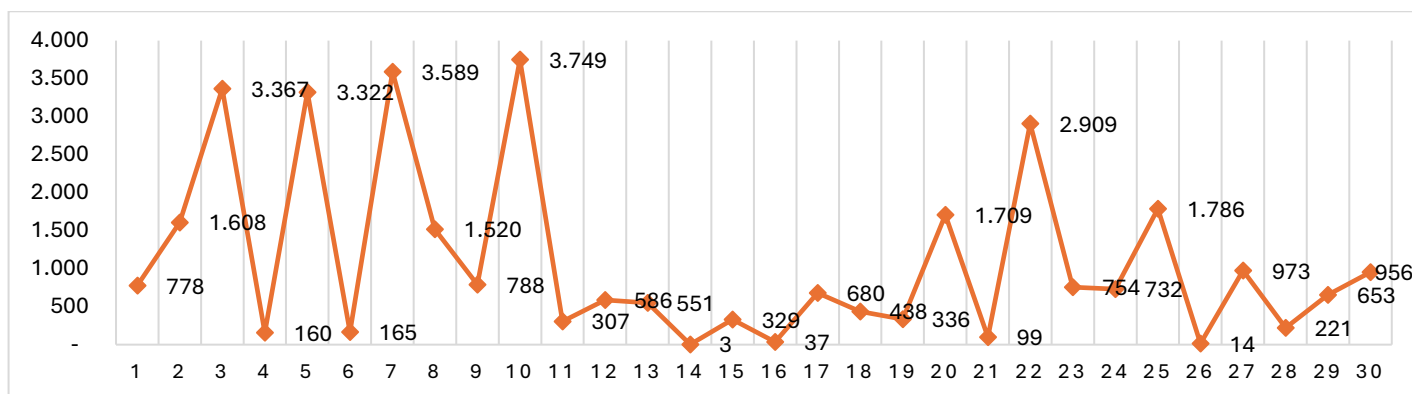
Graph 5 - Evolution of fire outbreaks in Bolivia Period: September 2024
