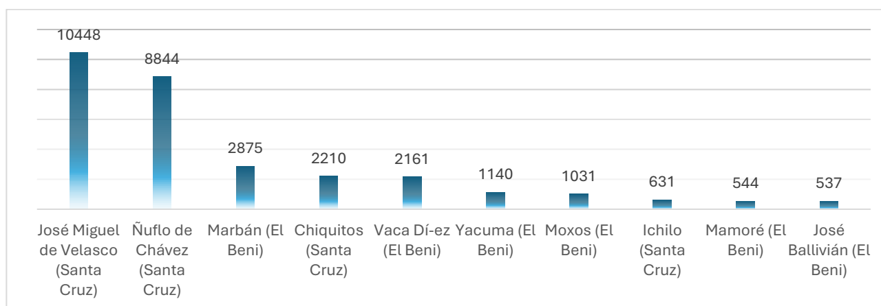
Graph 7 - Spotlights in a municipality in Bolivia Period: September 2024
