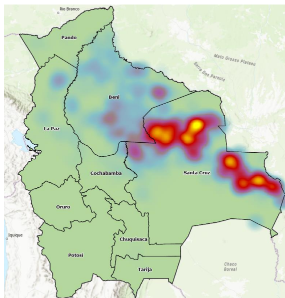
Heat map of fires in Bolivia Period: September 2024
