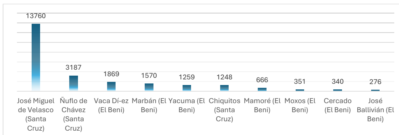
Graph 6 - Spotlights in a municipality in Bolivia Period: August 2024
