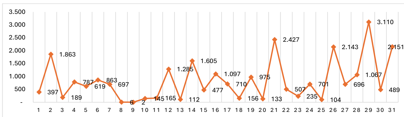
Graph 4 - Evolution of fire outbreaks Period: August 2024
